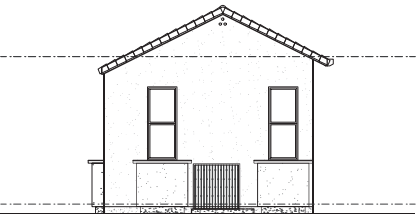
C REAR ELEVATION A2.2 1/4" = 1'-0"
