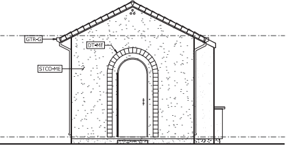
A FRONT ELEVATION A2.2 1/4" = 1'-0"
