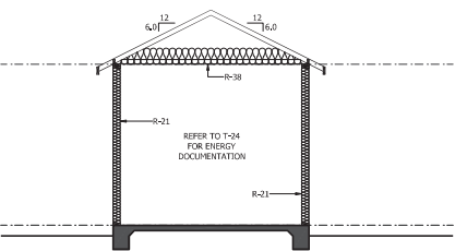
E SECTION A2.2 1/4" = 1'-0"
