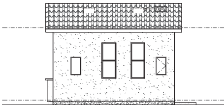
D LEFT ELEVATION A2.2 1/4" = 1'-0"
